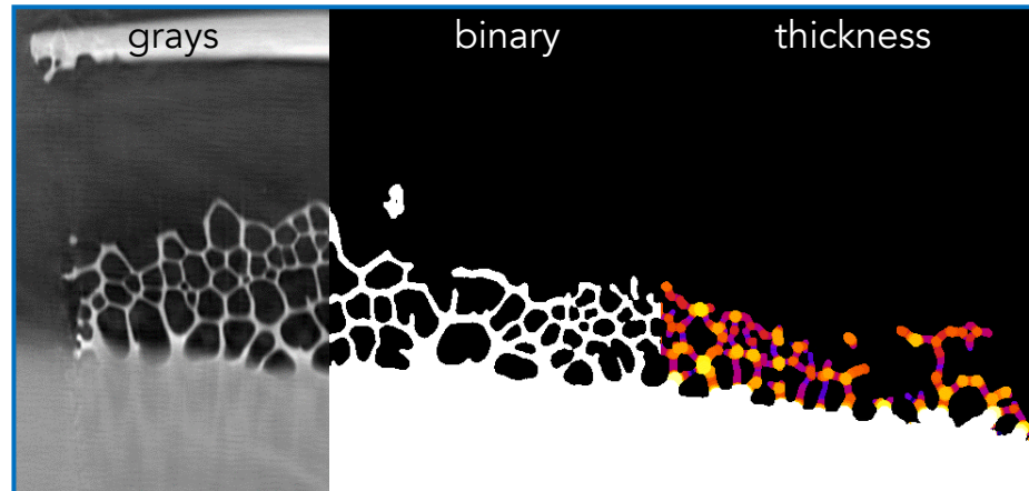
structure thickness
